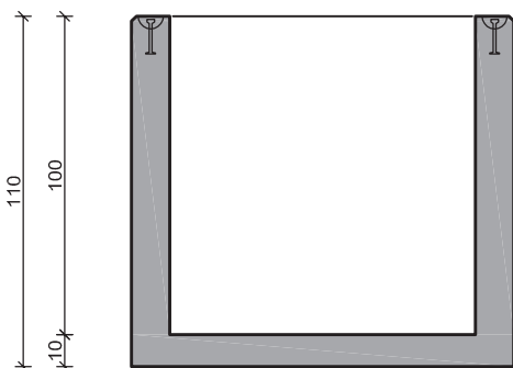
doorsnede put
