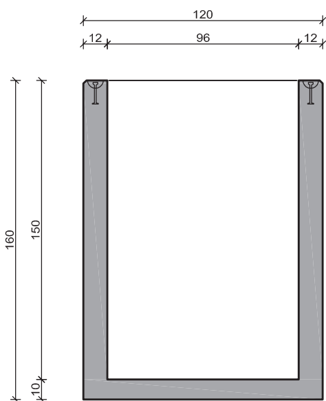
doorsnede put
