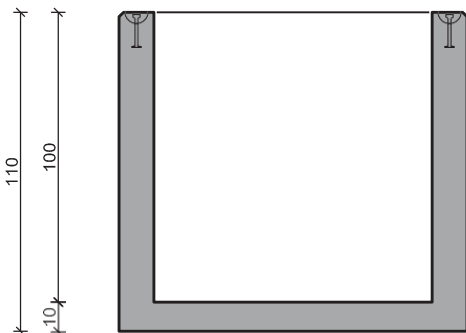
doorsnede put
