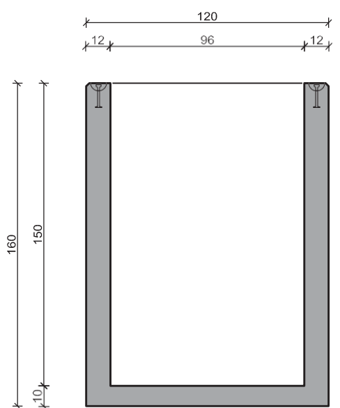
doorsnede put
